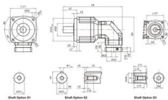
Dimensions (2-stage, Ratio i=15~200) / ABR Series
