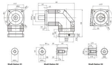
Dimensions (1-stage, Ratio i=3~20) / ABR Series
