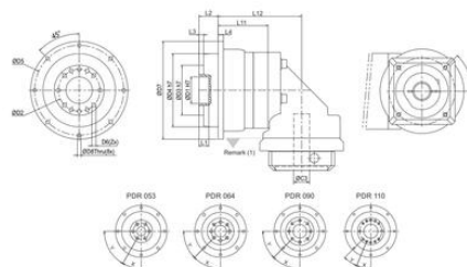
PDR Series Dimension
